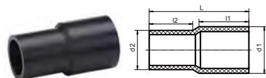
Reducer (WXGZ1100)
