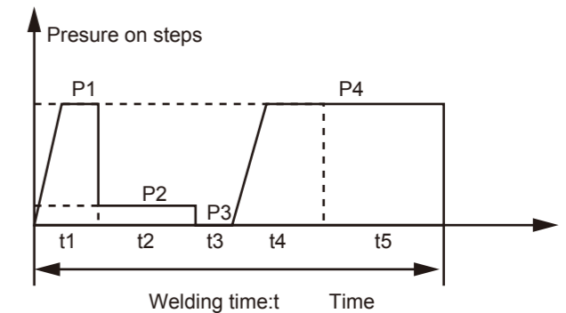
Figure 8.2.1.B Principle of Butt fusion of PE pipes
